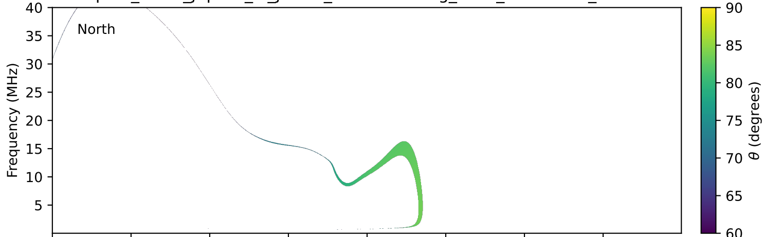
expres_earth_jupiter_io_jrm09_lossc-wid1deg_3kev_19960220_v11.cdf
