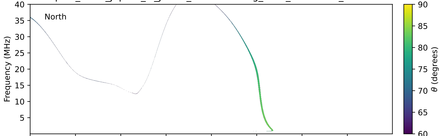
expres_earth_jupiter_io_jrm09_lossc-wid1deg_3kev_19960211_v11.cdf
