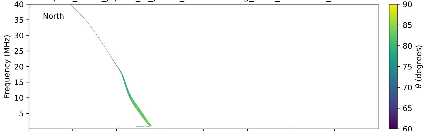
expres_earth_jupiter_io_jrm09_lossc-wid1deg_3kev_19960206_v11.cdf
