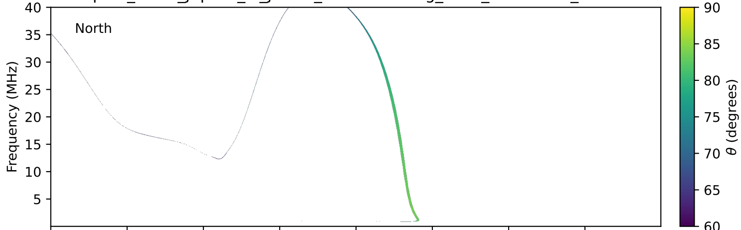
expres_earth_jupiter_io_jrm09_lossc-wid1deg_3kev_19960204_v11.cdf
