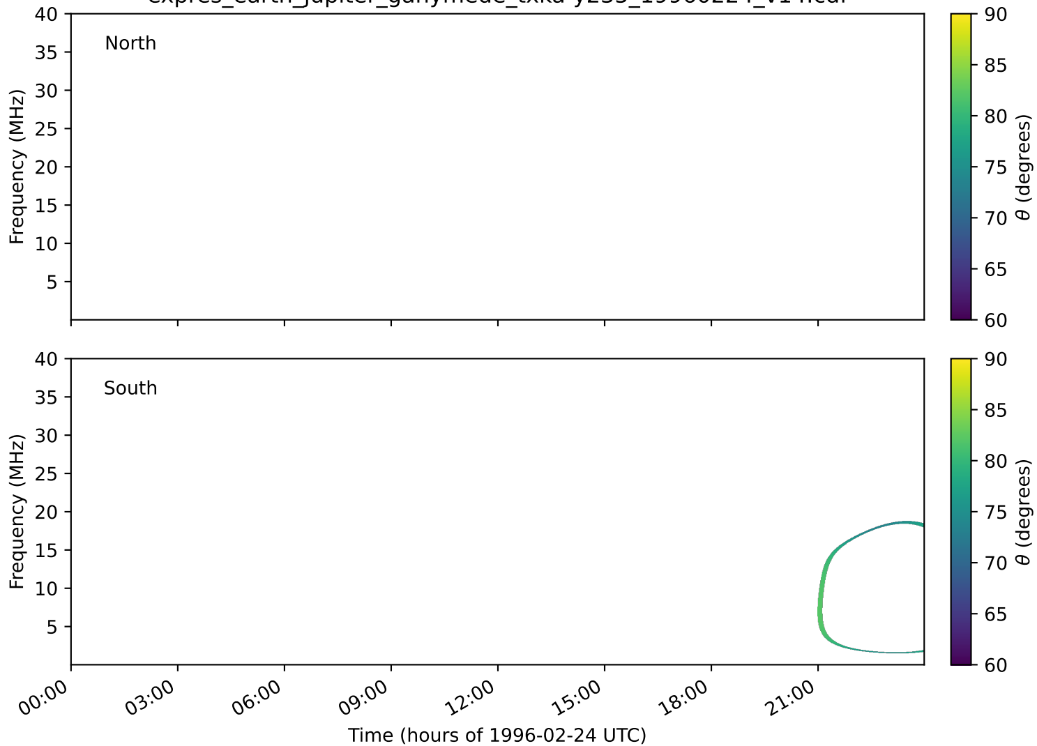
expres_earth_jupiter_ganymede_txka-y235_19960224_v14.cdf
