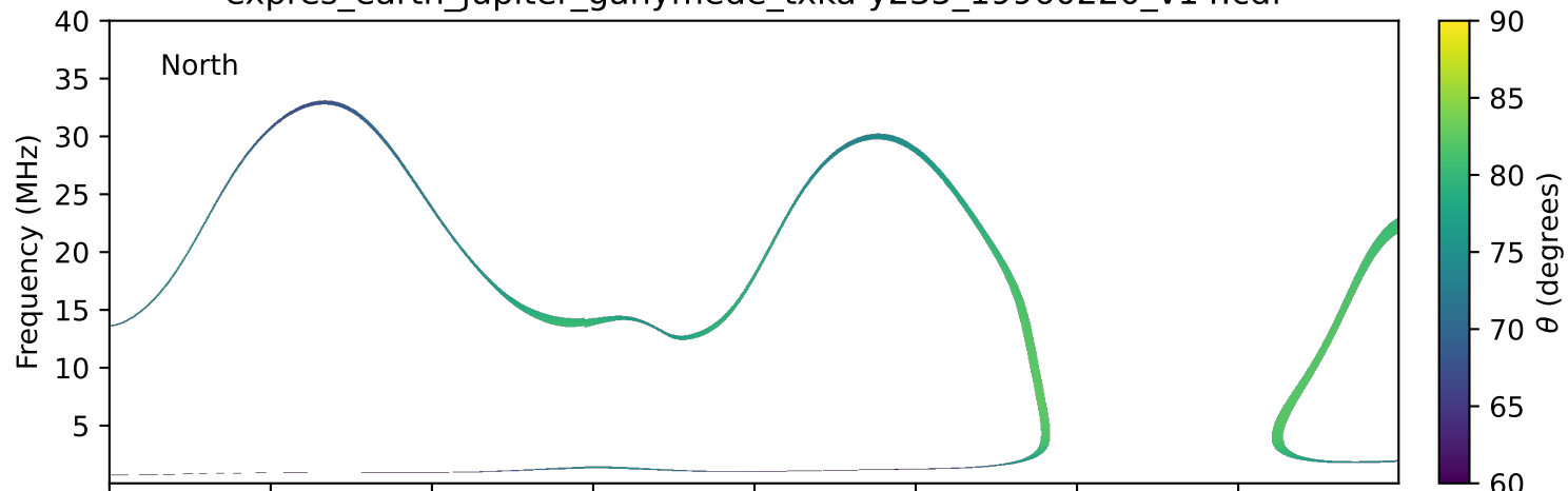
expres_earth_jupiter_ganymede_txka-y235_19960220_v14.cdf
