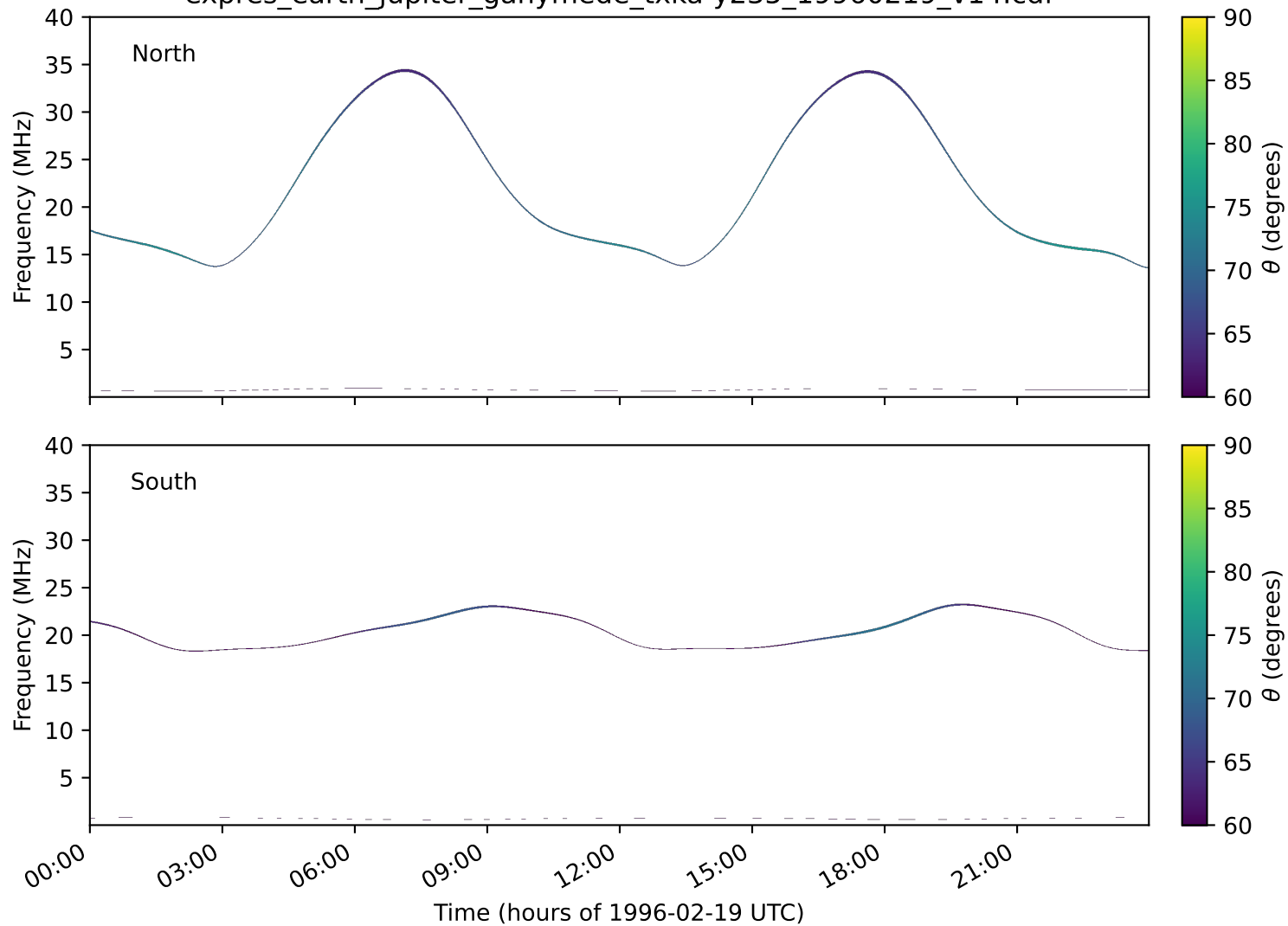
expres_earth_jupiter_ganymede_txka-y235_19960219_v14.cdf
