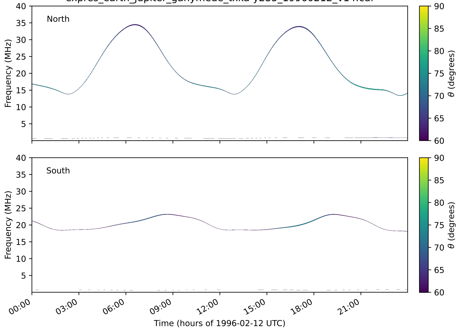
expres_earth_jupiter_ganymede_txka-y235_19960212_v14.cdf
