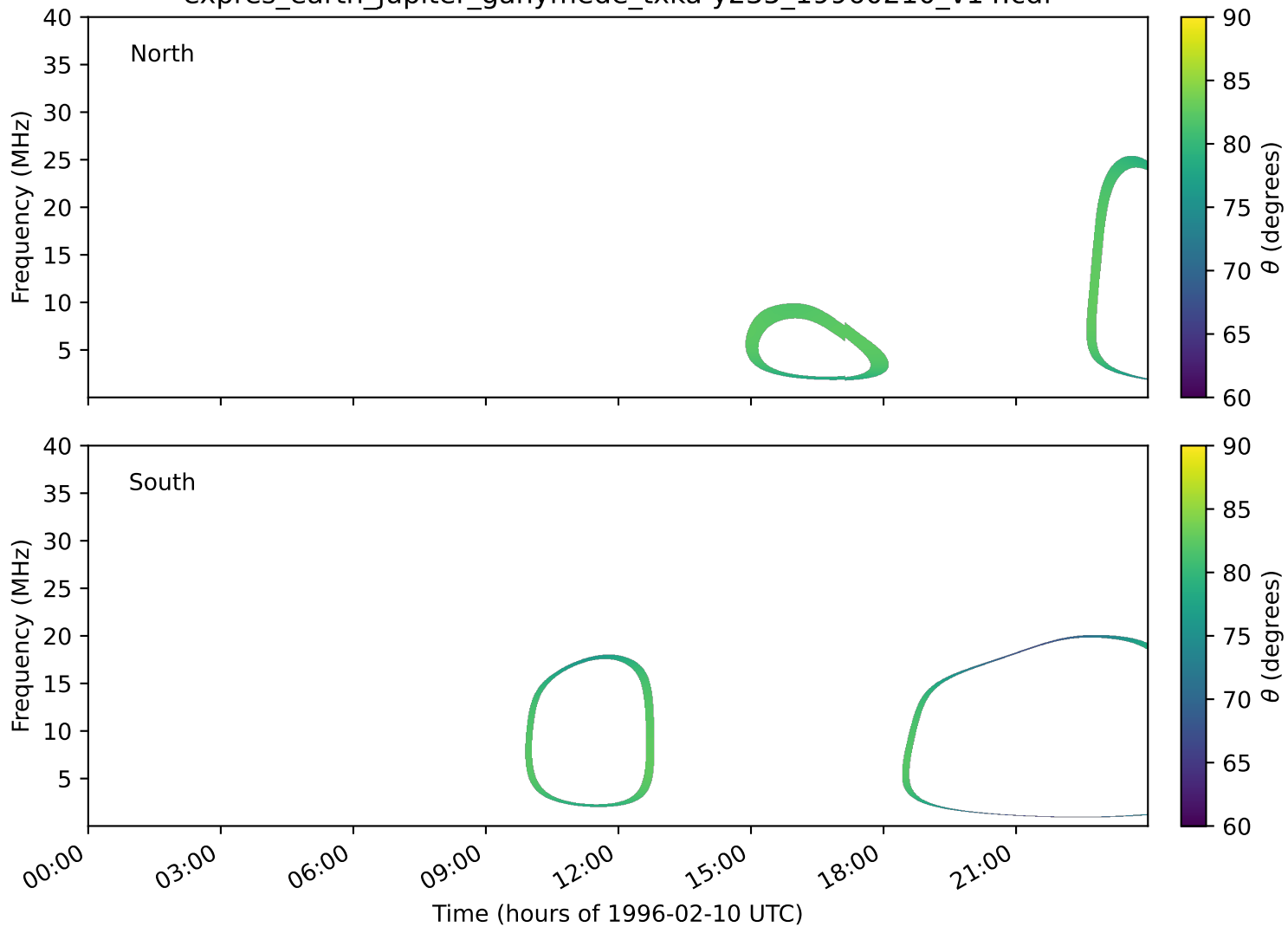
expres_earth_jupiter_ganymede_txka-y235_19960210_v14.cdf
