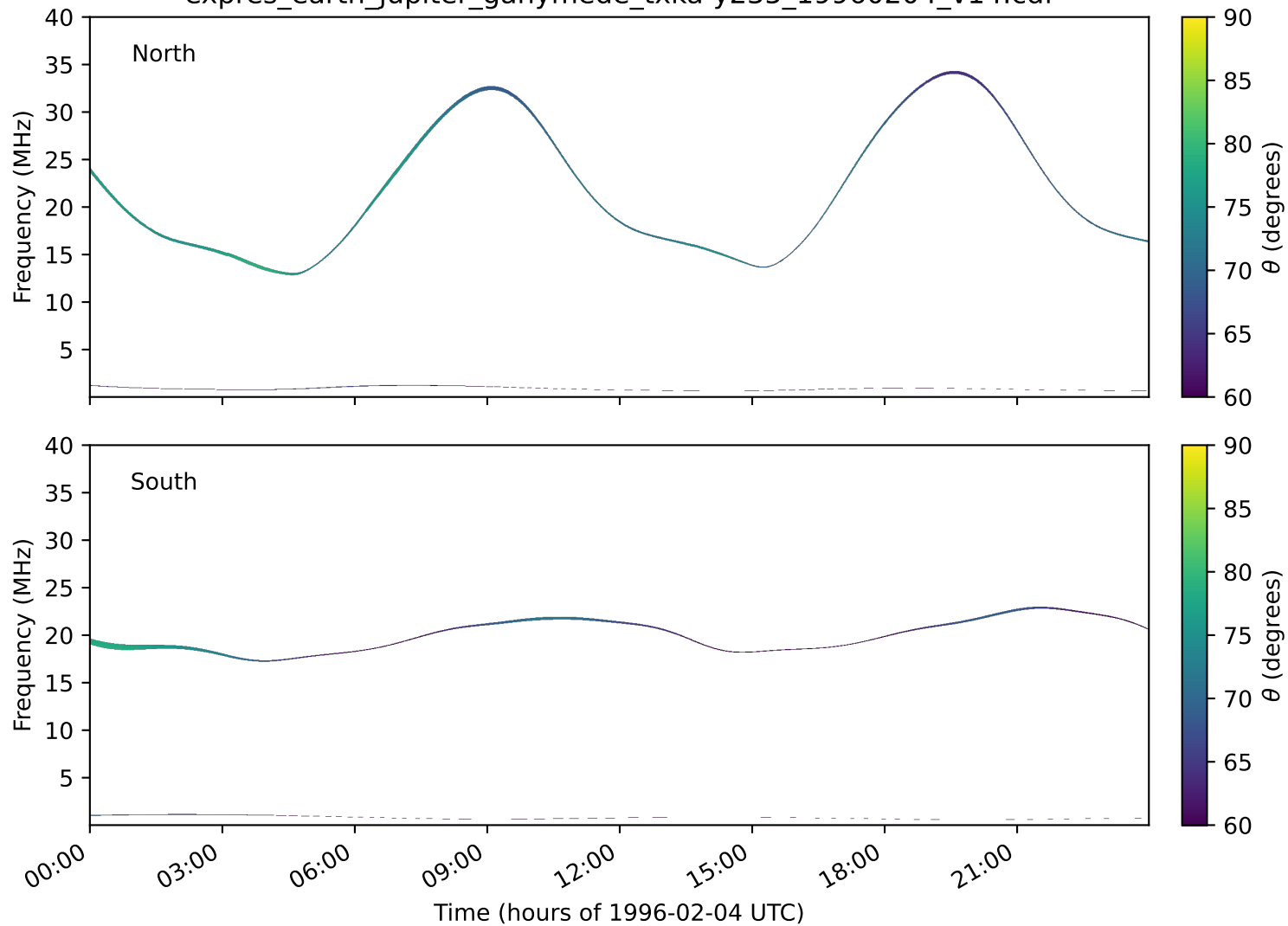
expres_earth_jupiter_ganymede_txka-y235_19960204_v14.cdf
