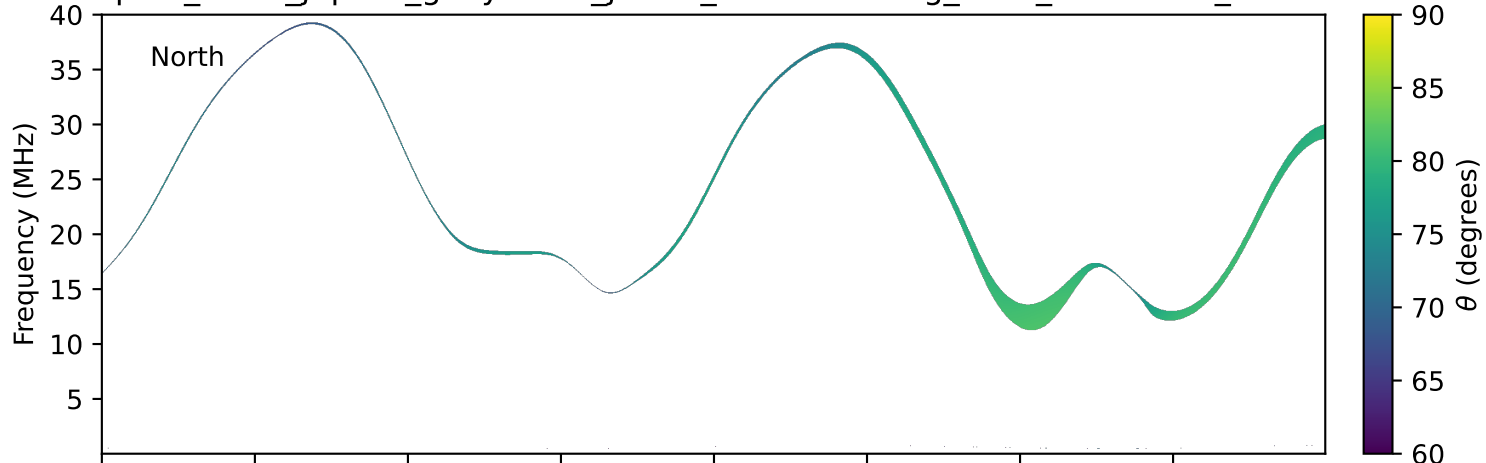
expres_earth_jupiter_ganymede_jrm33_lossc-wid1deg_3kev_19960220_v11.cdf
