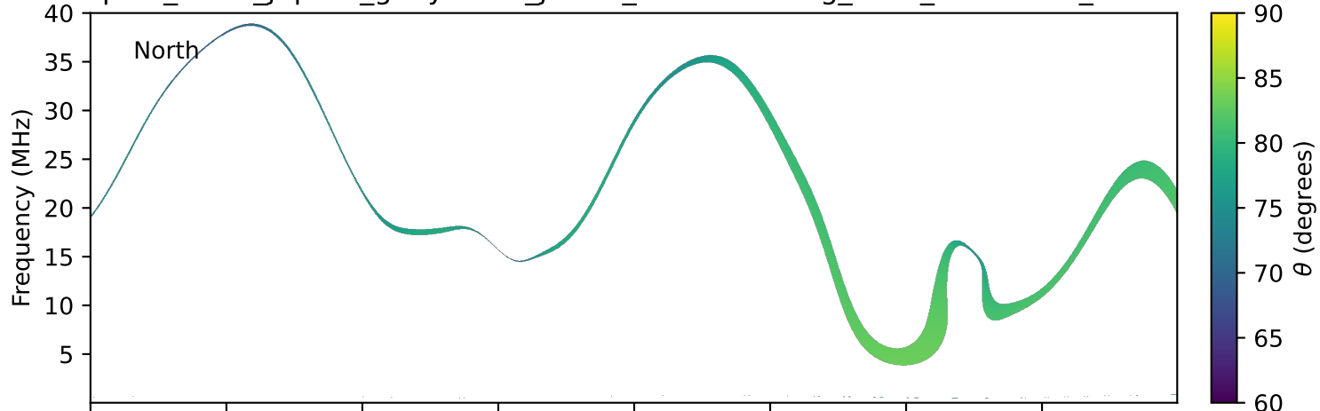
expres_earth_jupiter_ganymede_jrm33_lossc-wid1deg_3kev_19960213_v11.cdf
