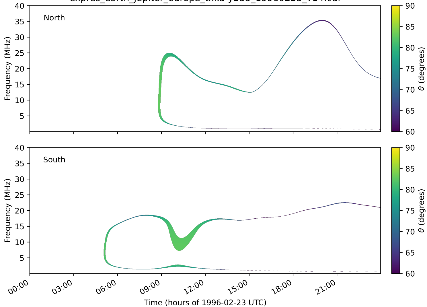
expres_earth_jupiter_europa_txka-y235_19960223_v14.cdf
