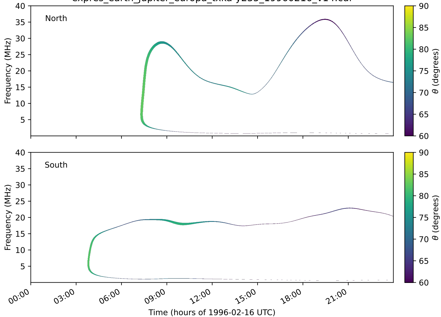
expres_earth_jupiter_europa_txka-y235_19960216_v14.cdf
