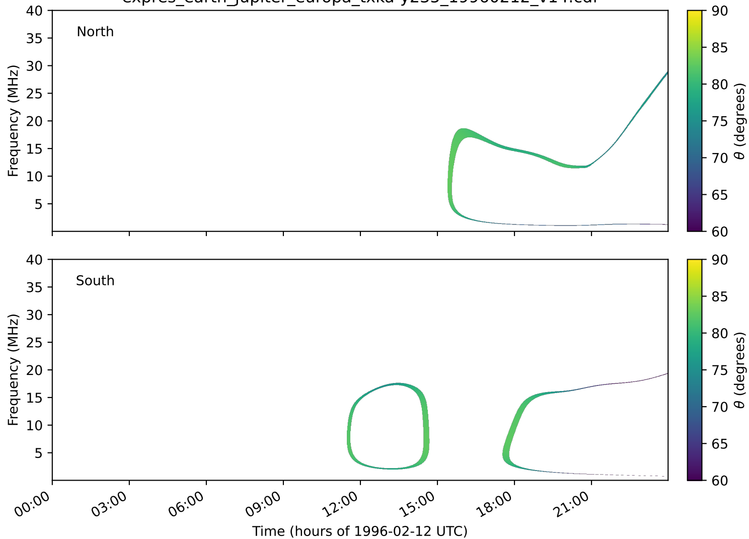
expres_earth_jupiter_europa_txka-y235_19960212_v14.cdf
