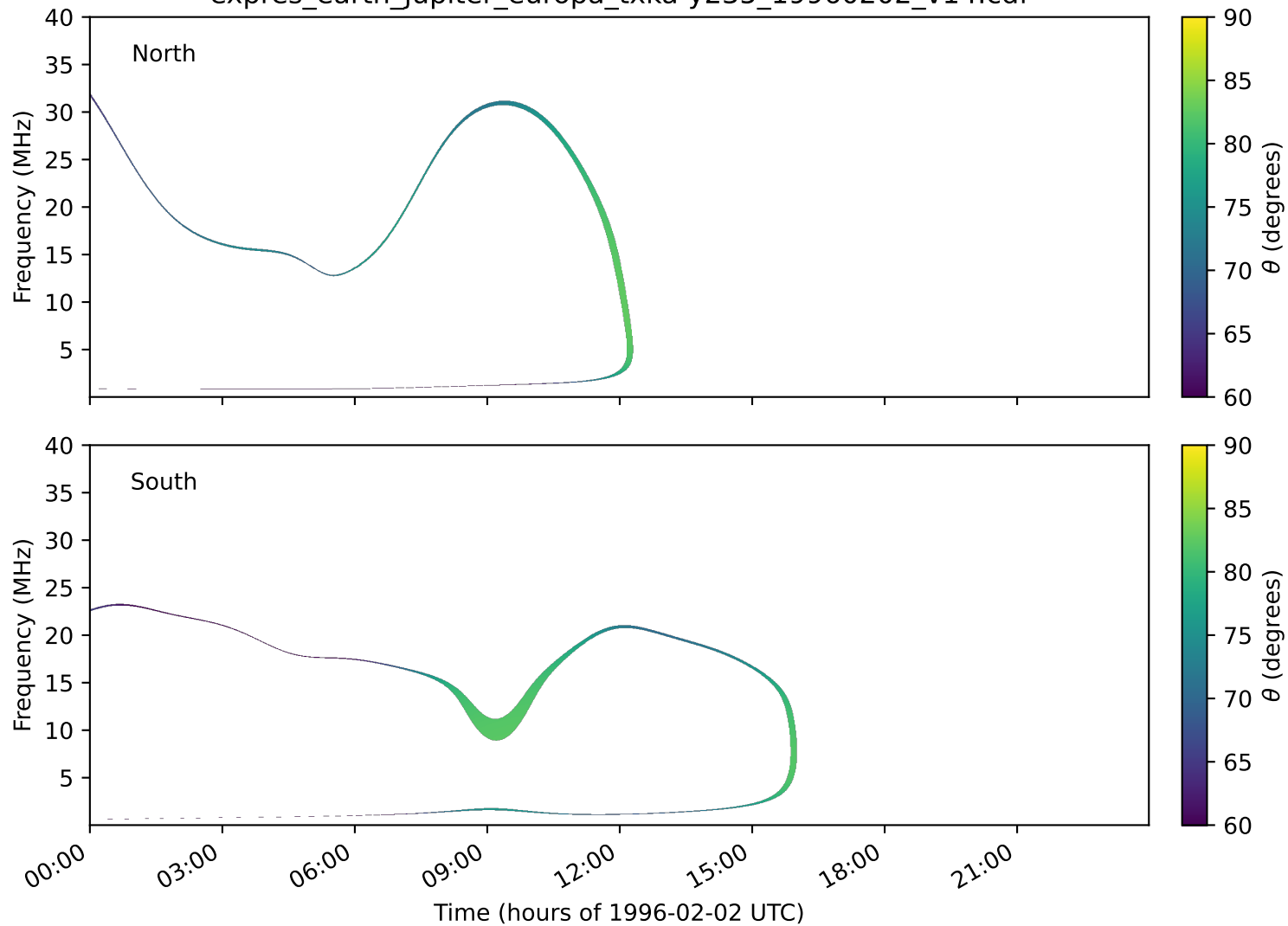
expres_earth_jupiter_europa_txka-y235_19960202_v14.cdf
