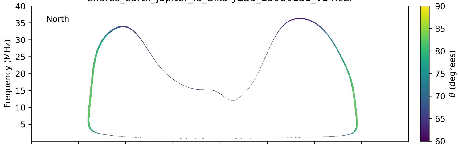
expres_earth_jupiter_io_txka-y235_19960131_v14.cdf
