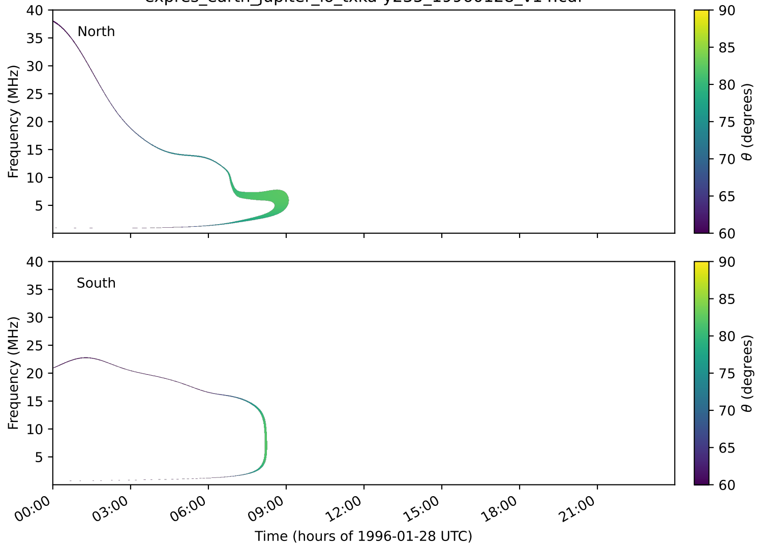
expres_earth_jupiter_io_txka-y235_19960128_v14.cdf
