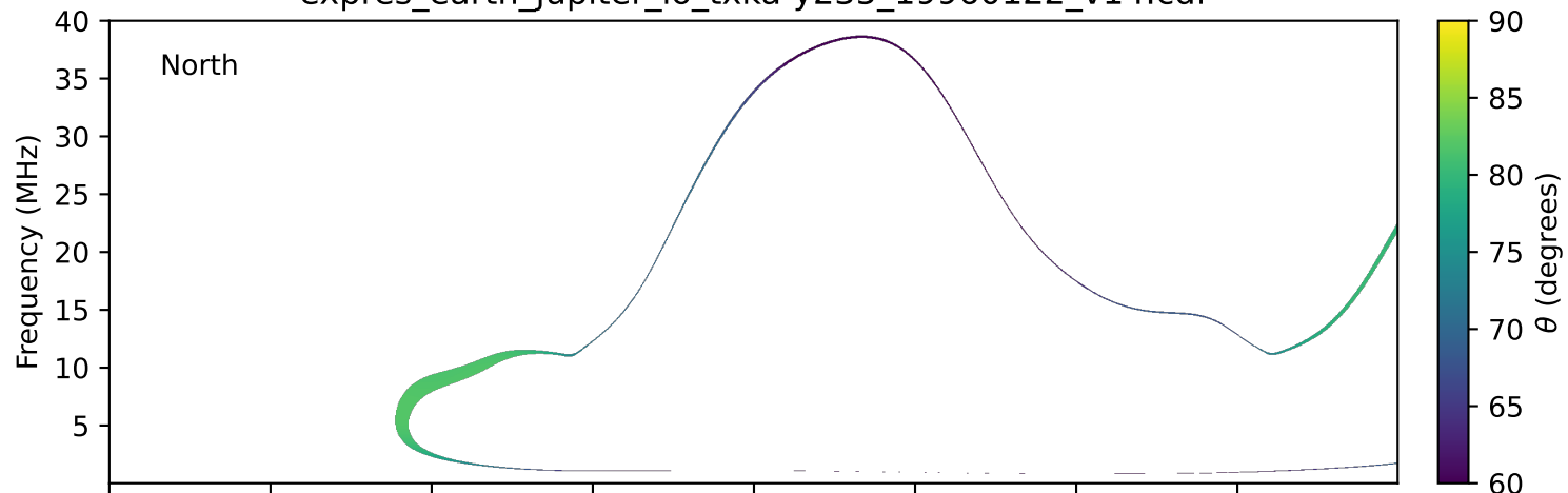
expres_earth_jupiter_io_txka-y235_19960122_v14.cdf
