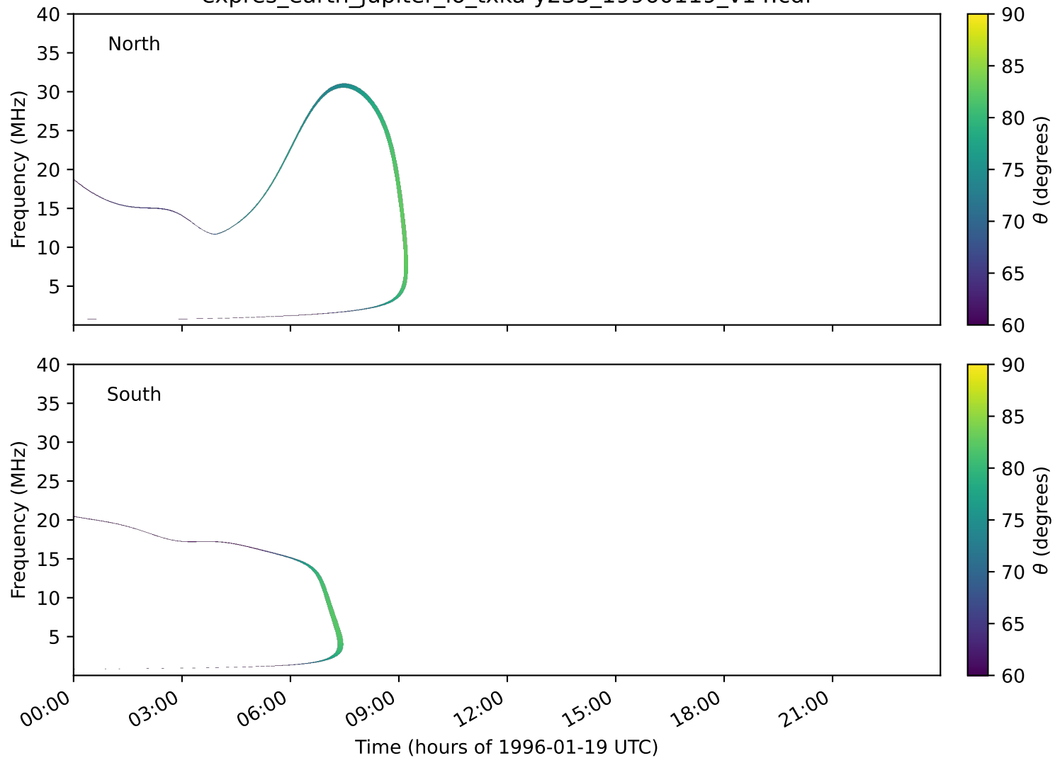
expres_earth_jupiter_io_txka-y235_19960119_v14.cdf
