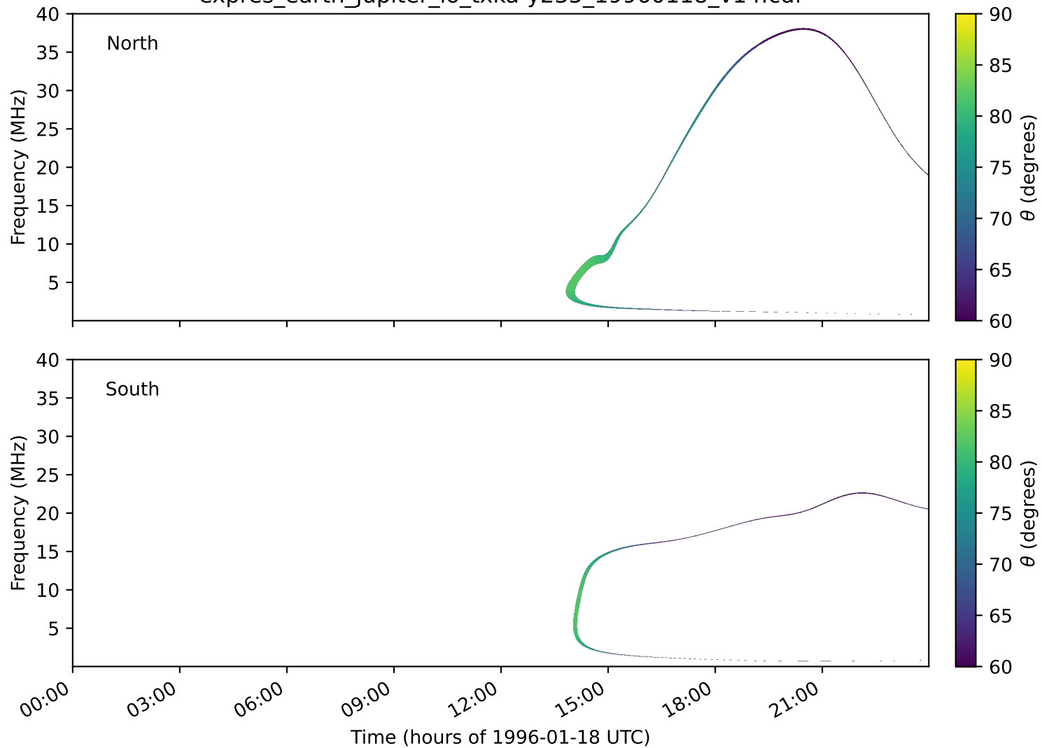
expres_earth_jupiter_io_txka-y235_19960118_v14.cdf
