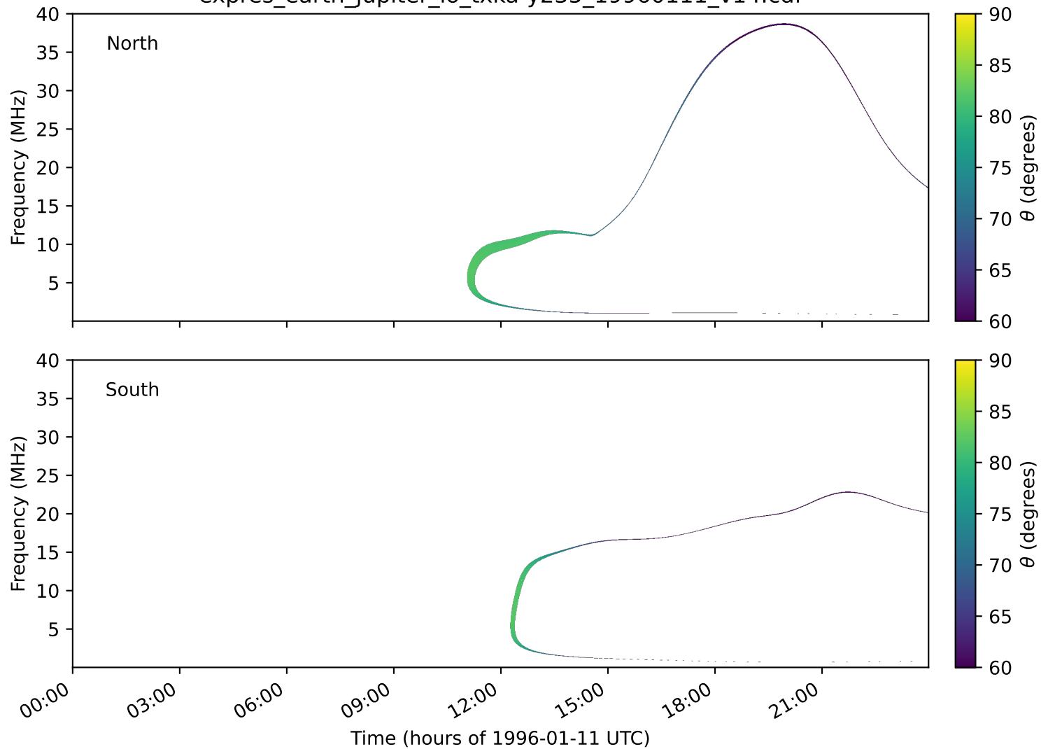
expres_earth_jupiter_io_txka-y235_19960111_v14.cdf
