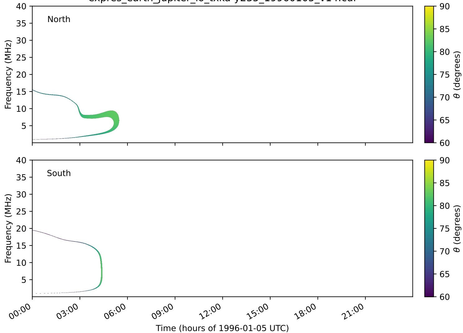
expres_earth_jupiter_io_txka-y235_19960105_v14.cdf
