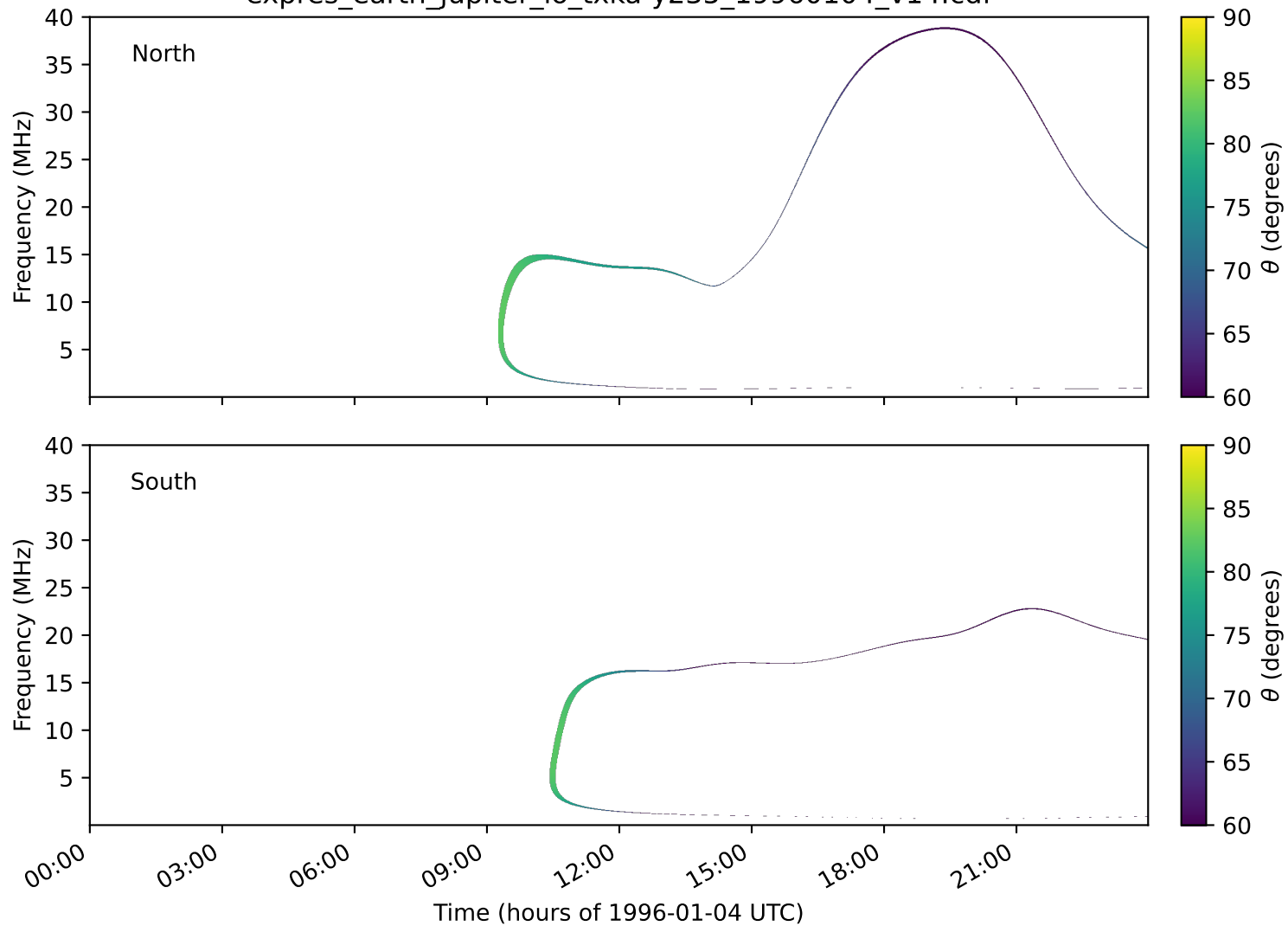
expres_earth_jupiter_io_txka-y235_19960104_v14.cdf
