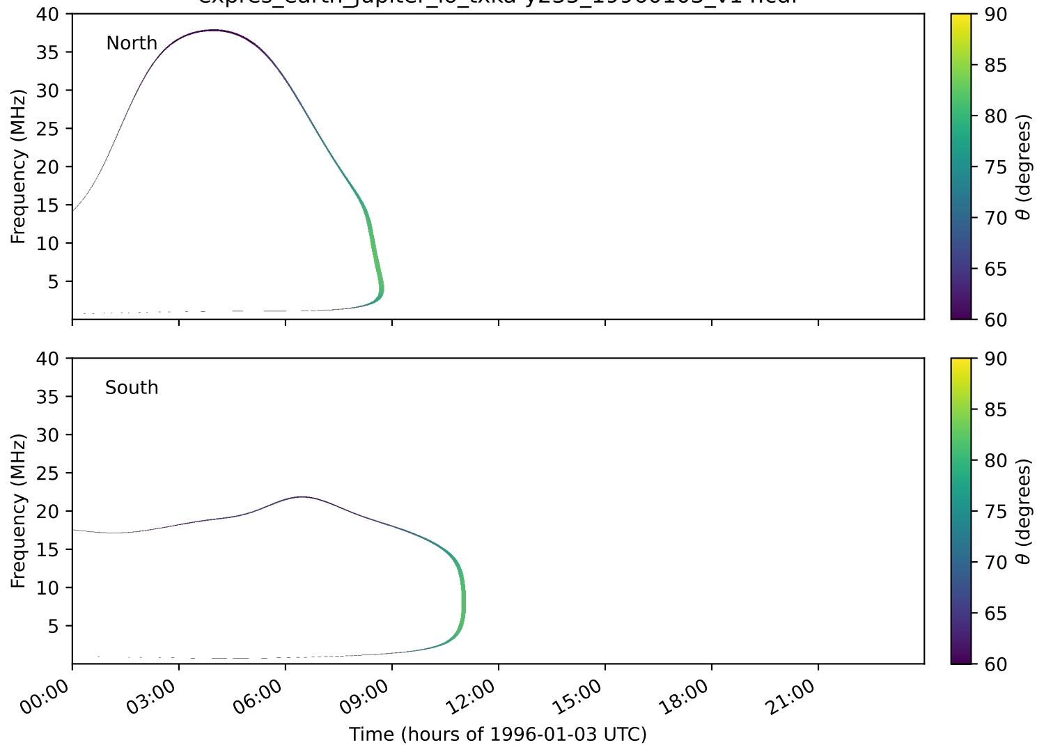
expres_earth_jupiter_io_txka-y235_19960103_v14.cdf
