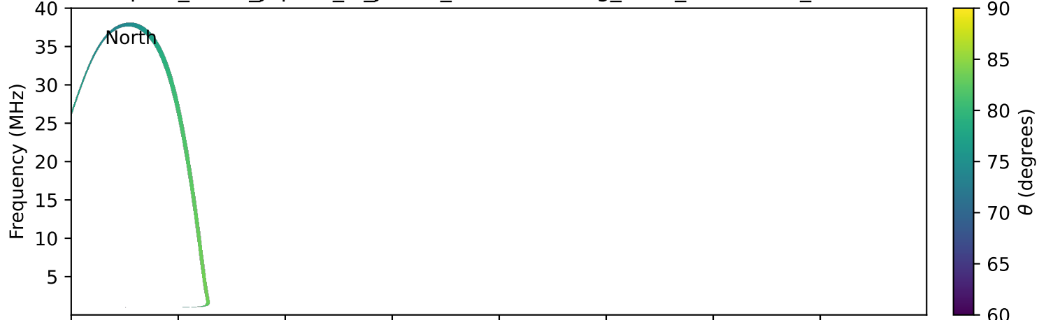
expres_earth_jupiter_io_jrm33_lossc-wid1deg_3kev_19960130_v11.cdf
