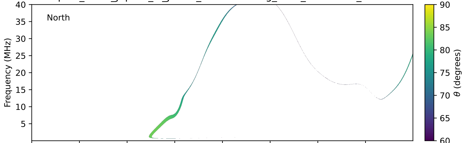
expres_earth_jupiter_io_jrm33_lossc-wid1deg_3kev_19960129_v11.cdf
