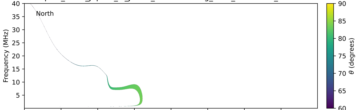
expres_earth_jupiter_io_jrm33_lossc-wid1deg_3kev_19960128_v11.cdf
