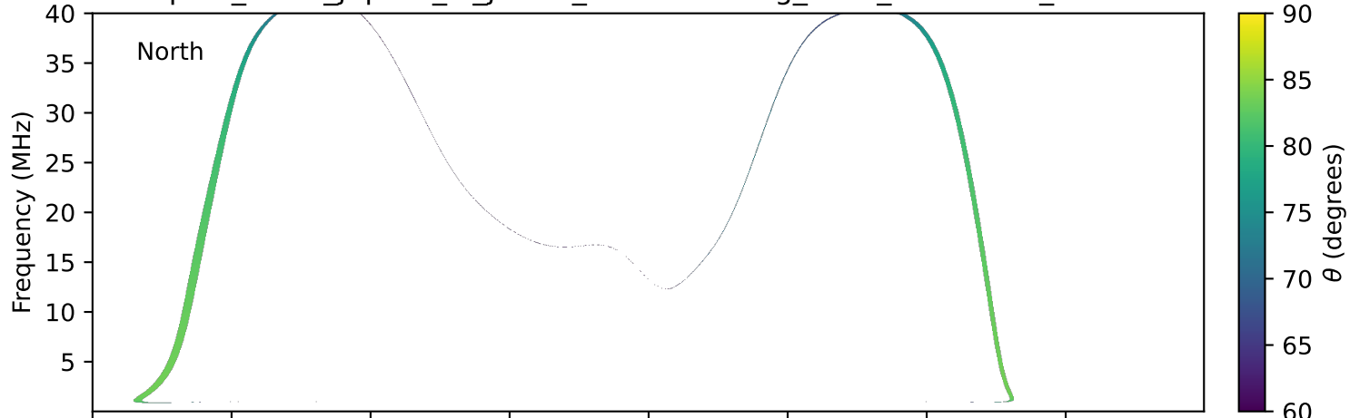
expres_earth_jupiter_io_jrm33_lossc-wid1deg_3kev_19960124_v11.cdf
