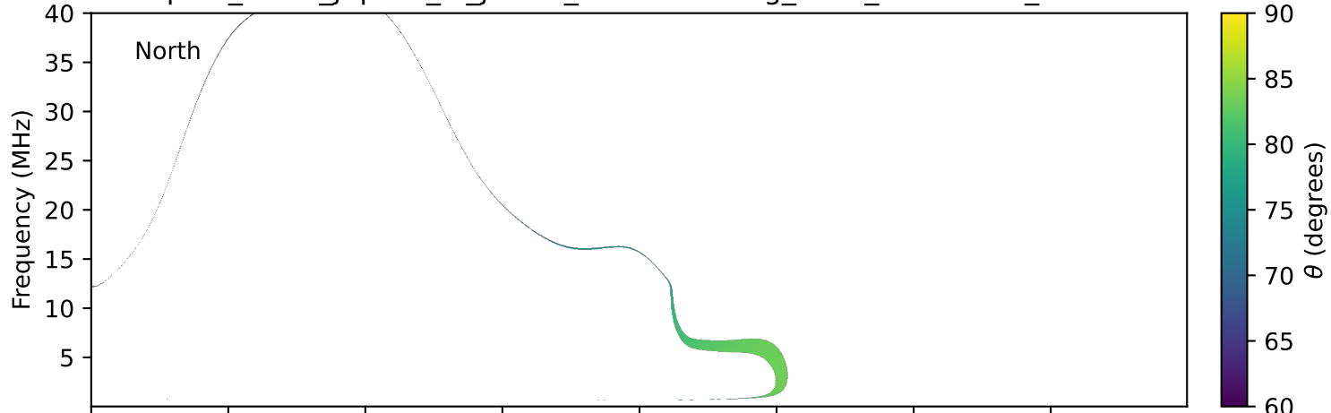
expres_earth_jupiter_io_jrm33_lossc-wid1deg_3kev_19960117_v11.cdf
