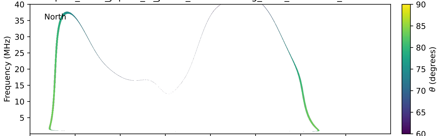
expres_earth_jupiter_io_jrm33_lossc-wid1deg_3kev_19960115_v11.cdf
