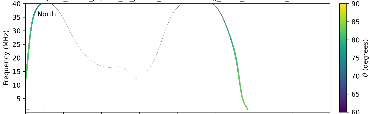
expres_earth_jupiter_io_jrm33_lossc-wid1deg_3kev_19960108_v11.cdf
