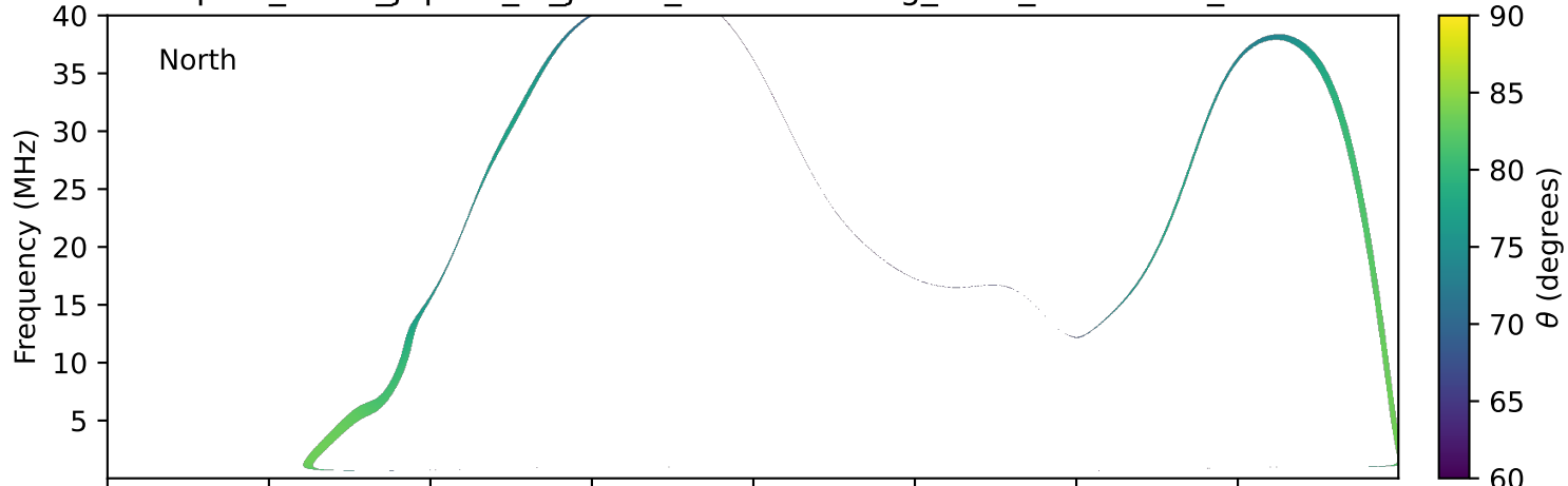
expres_earth_jupiter_io_jrm33_lossc-wid1deg_3kev_19960106_v11.cdf
