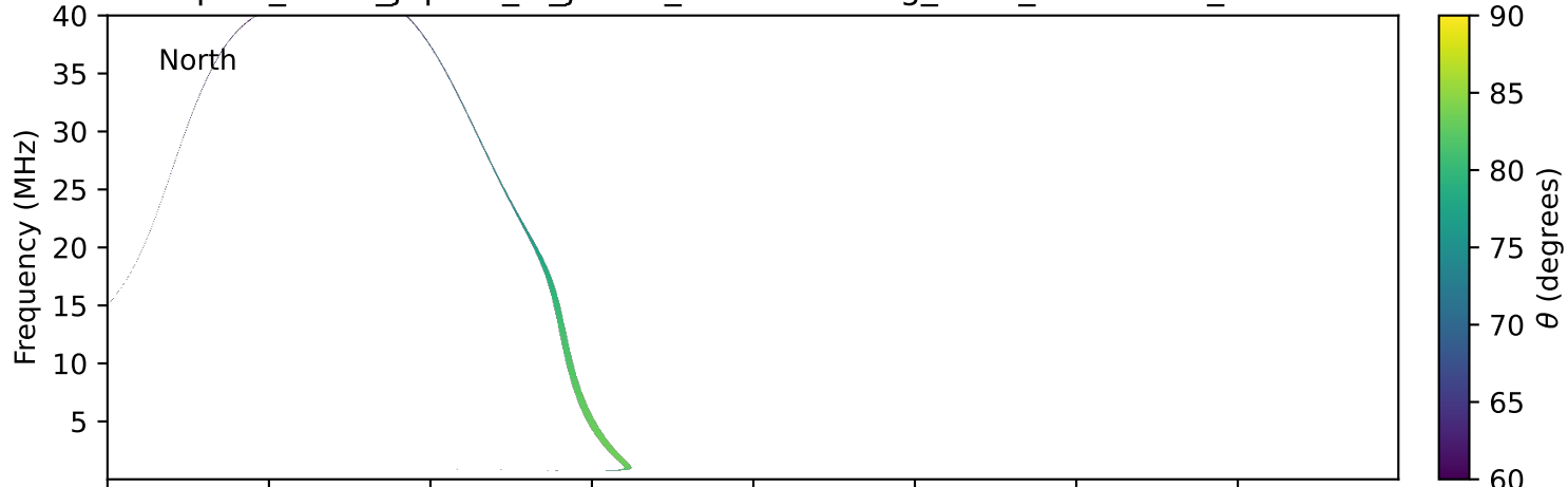
expres_earth_jupiter_io_jrm33_lossc-wid1deg_3kev_19960103_v11.cdf
