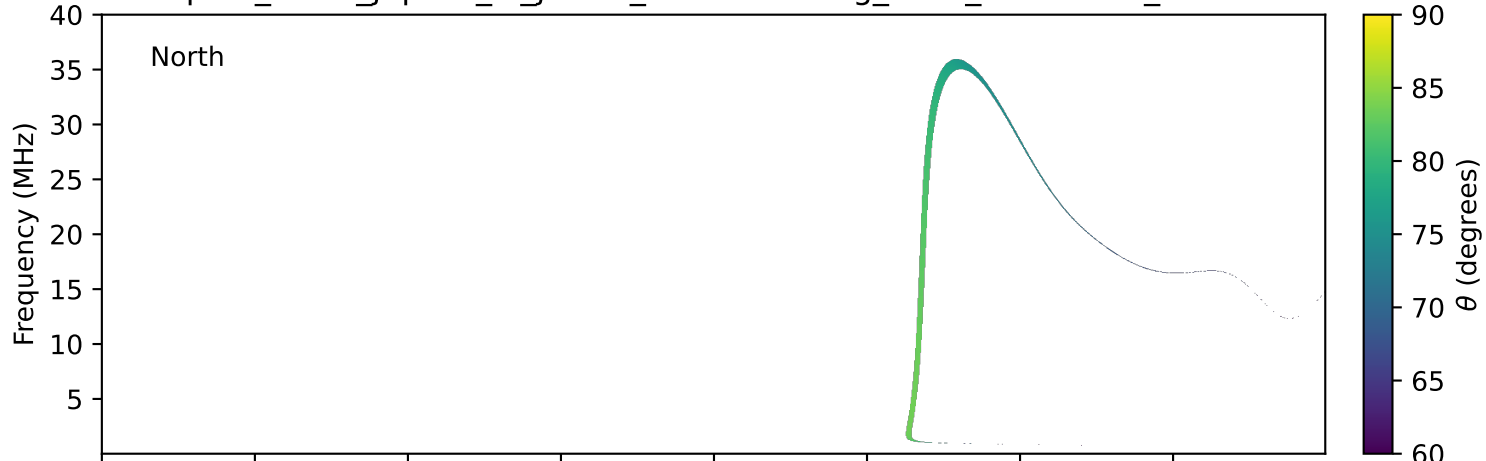
expres_earth_jupiter_io_jrm33_lossc-wid1deg_3kev_19960102_v11.cdf
