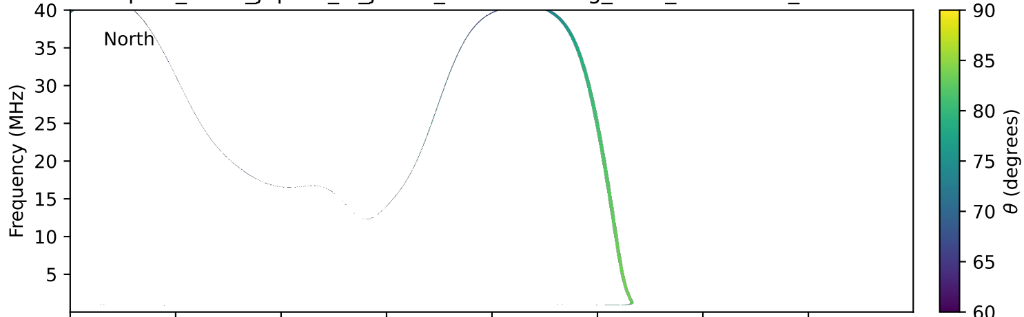
expres_earth_jupiter_io_jrm33_lossc-wid1deg_3kev_19960101_v11.cdf
