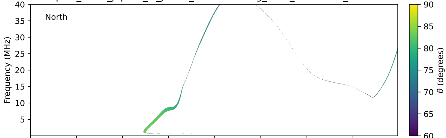
expres_earth_jupiter_io_jrm09_lossc-wid1deg_3kev_19960129_v11.cdf
