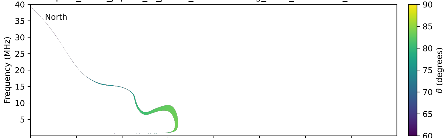
expres_earth_jupiter_io_jrm09_lossc-wid1deg_3kev_19960128_v11.cdf
