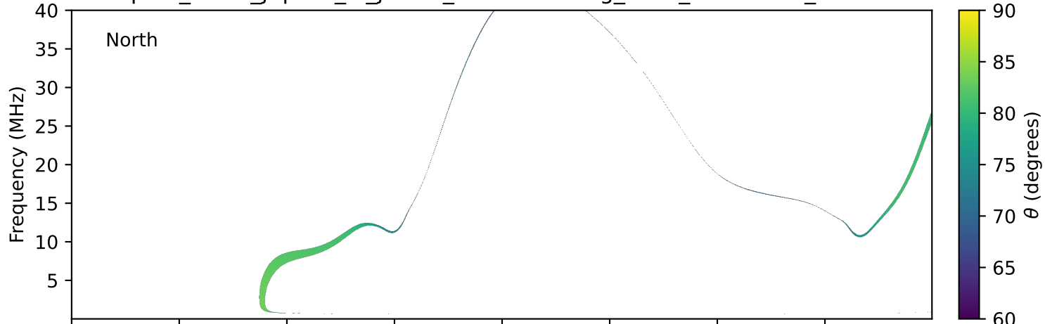
expres_earth_jupiter_io_jrm09_lossc-wid1deg_3kev_19960122_v11.cdf
