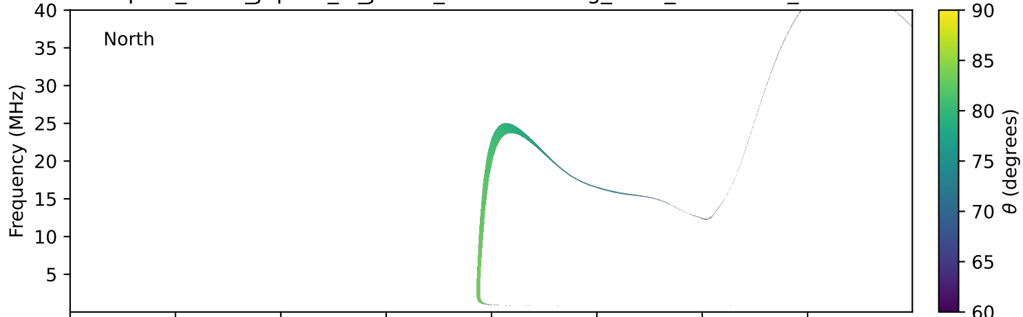
expres_earth_jupiter_io_jrm09_lossc-wid1deg_3kev_19960120_v11.cdf
