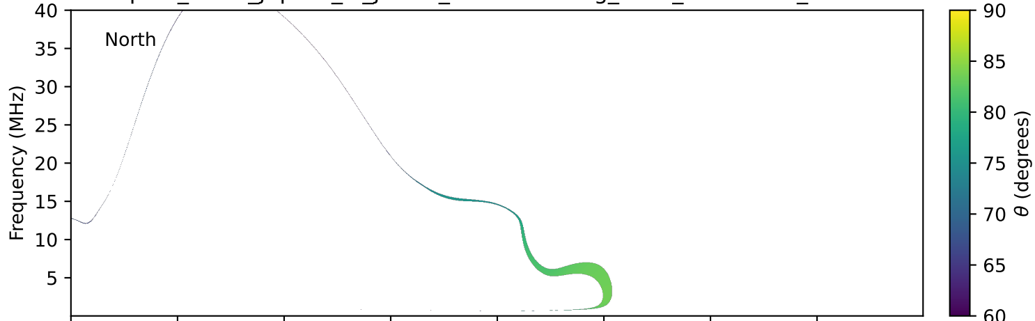
expres_earth_jupiter_io_jrm09_lossc-wid1deg_3kev_19960117_v11.cdf
