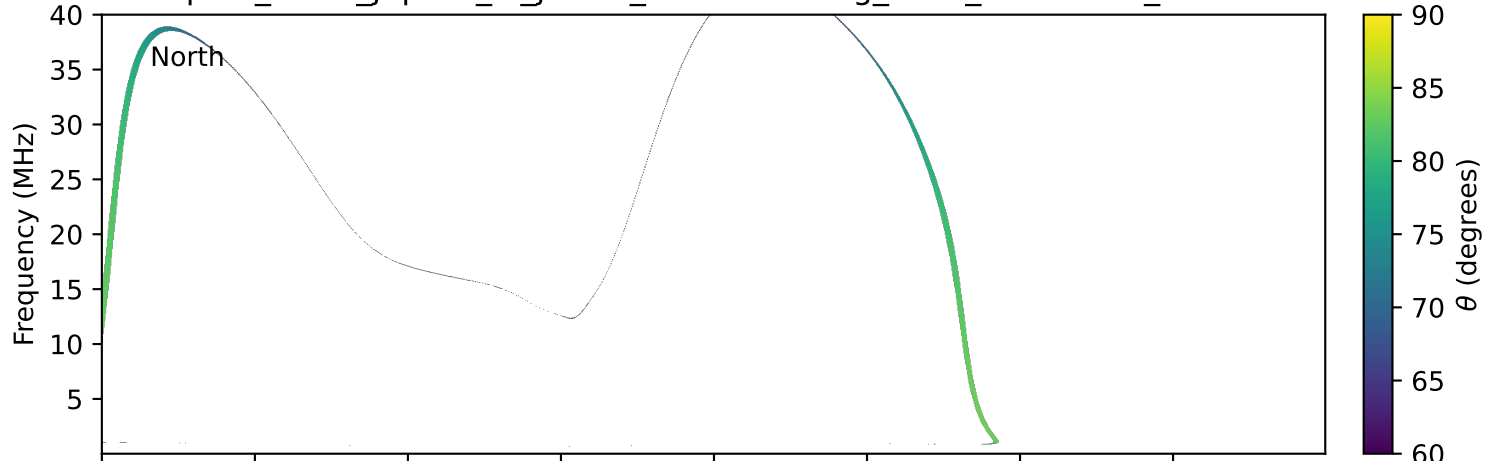
expres_earth_jupiter_io_jrm09_lossc-wid1deg_3kev_19960108_v11.cdf
