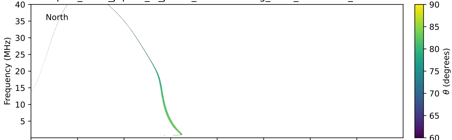
expres_earth_jupiter_io_jrm09_lossc-wid1deg_3kev_19960103_v11.cdf
