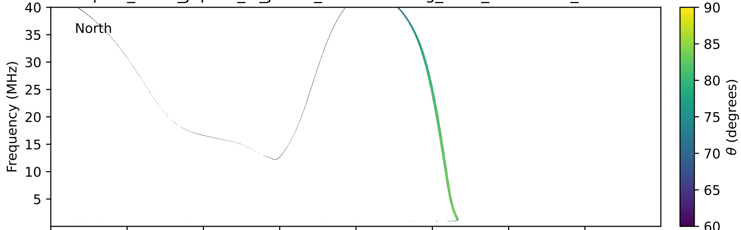
expres_earth_jupiter_io_jrm09_lossc-wid1deg_3kev_19960101_v11.cdf
