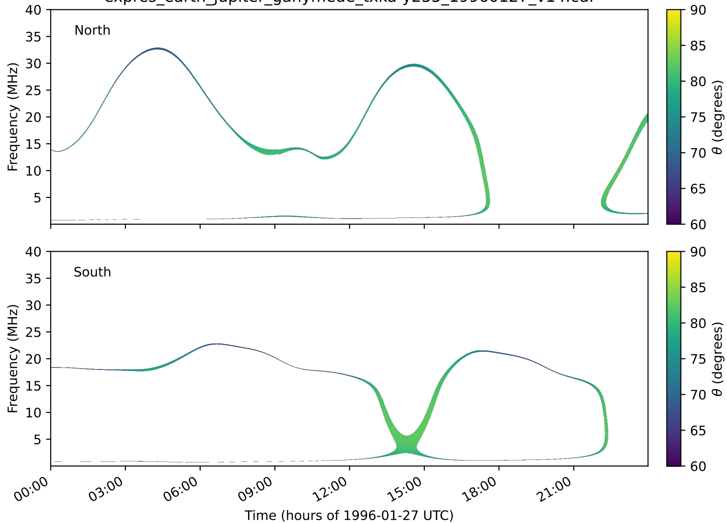
expres_earth_jupiter_ganymede_txka-y235_19960127_v14.cdf
