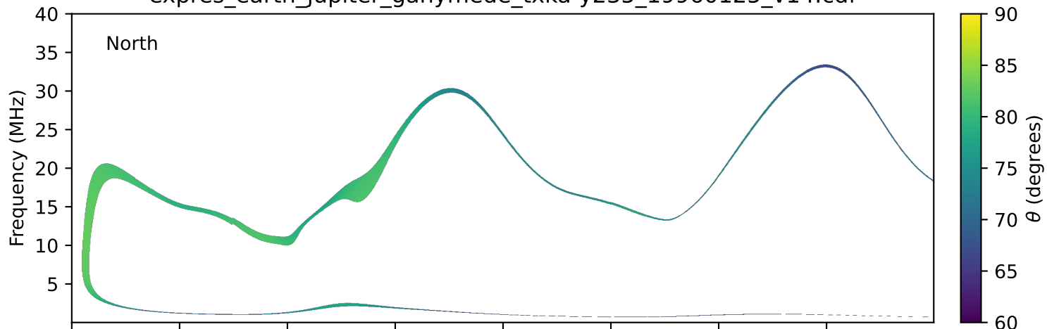
expres_earth_jupiter_ganymede_txka-y235_19960125_v14.cdf
