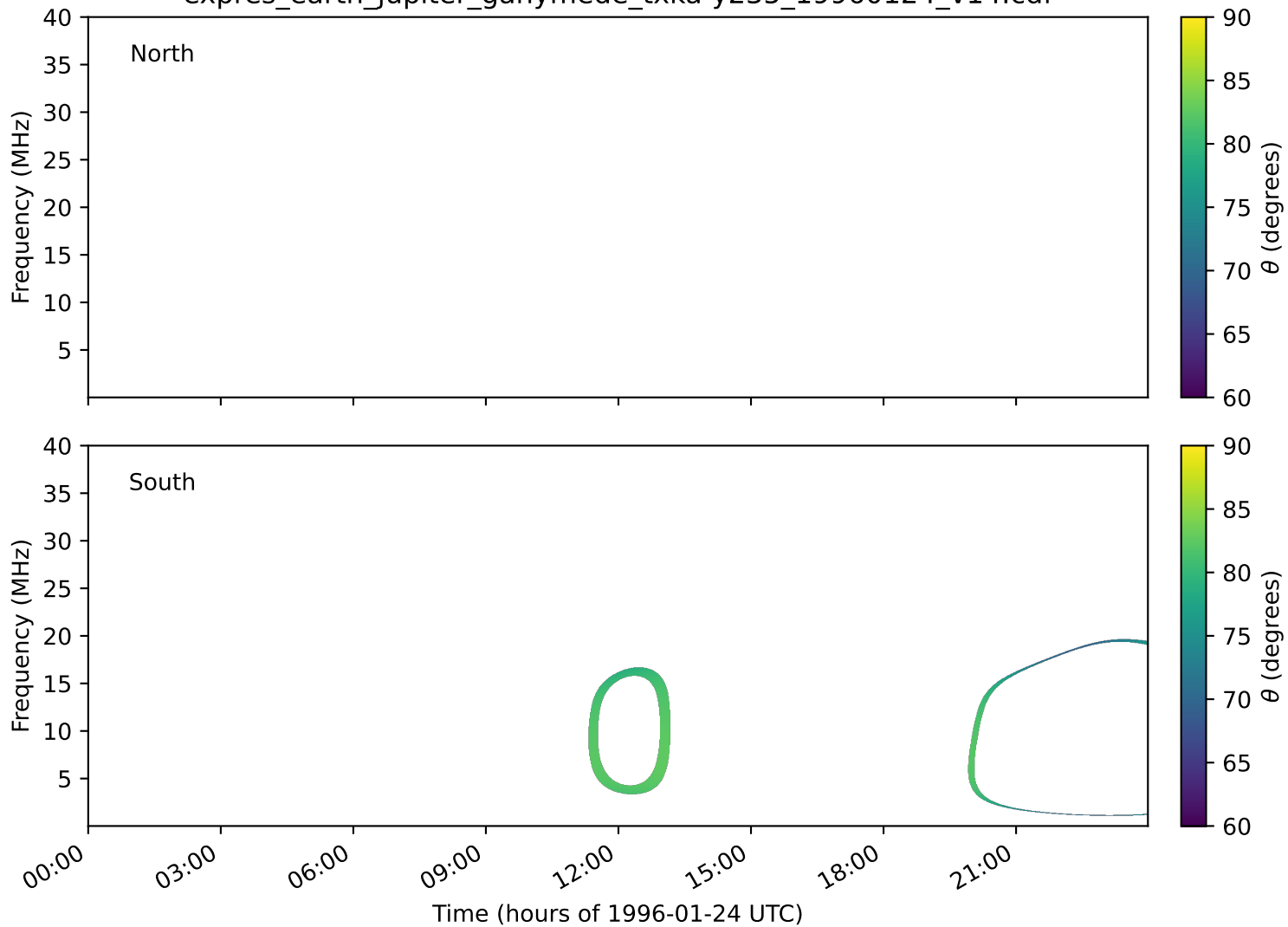
expres_earth_jupiter_ganymede_txka-y235_19960124_v14.cdf
