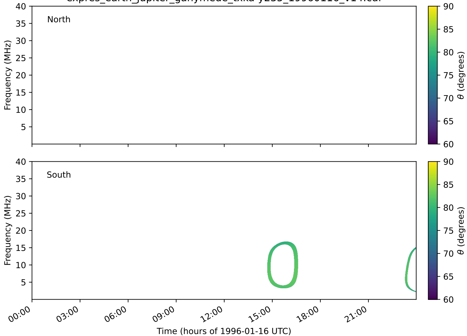
expres_earth_jupiter_ganymede_txka-y235_19960116_v14.cdf
