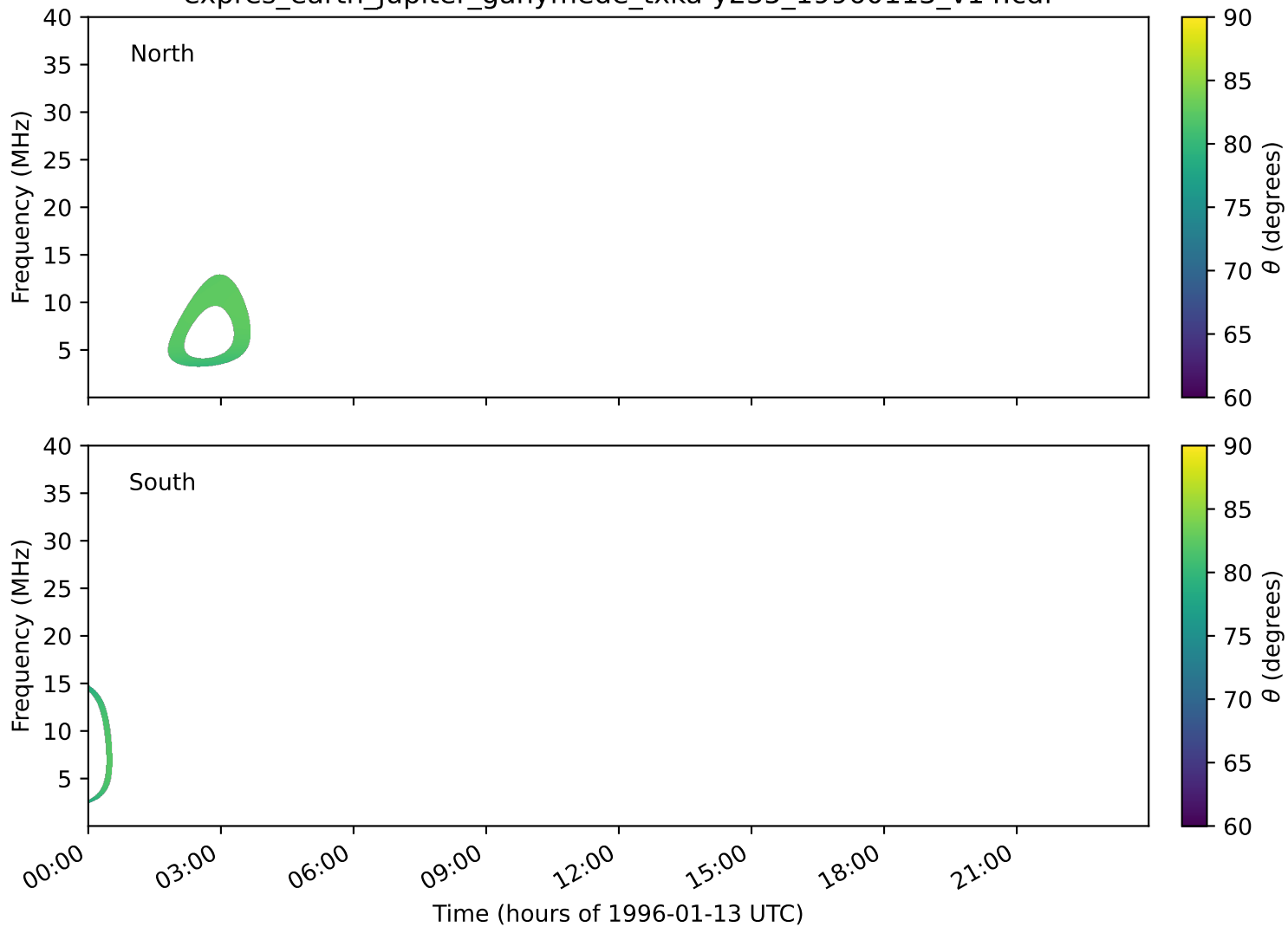
expres_earth_jupiter_ganymede_txka-y235_19960113_v14.cdf
