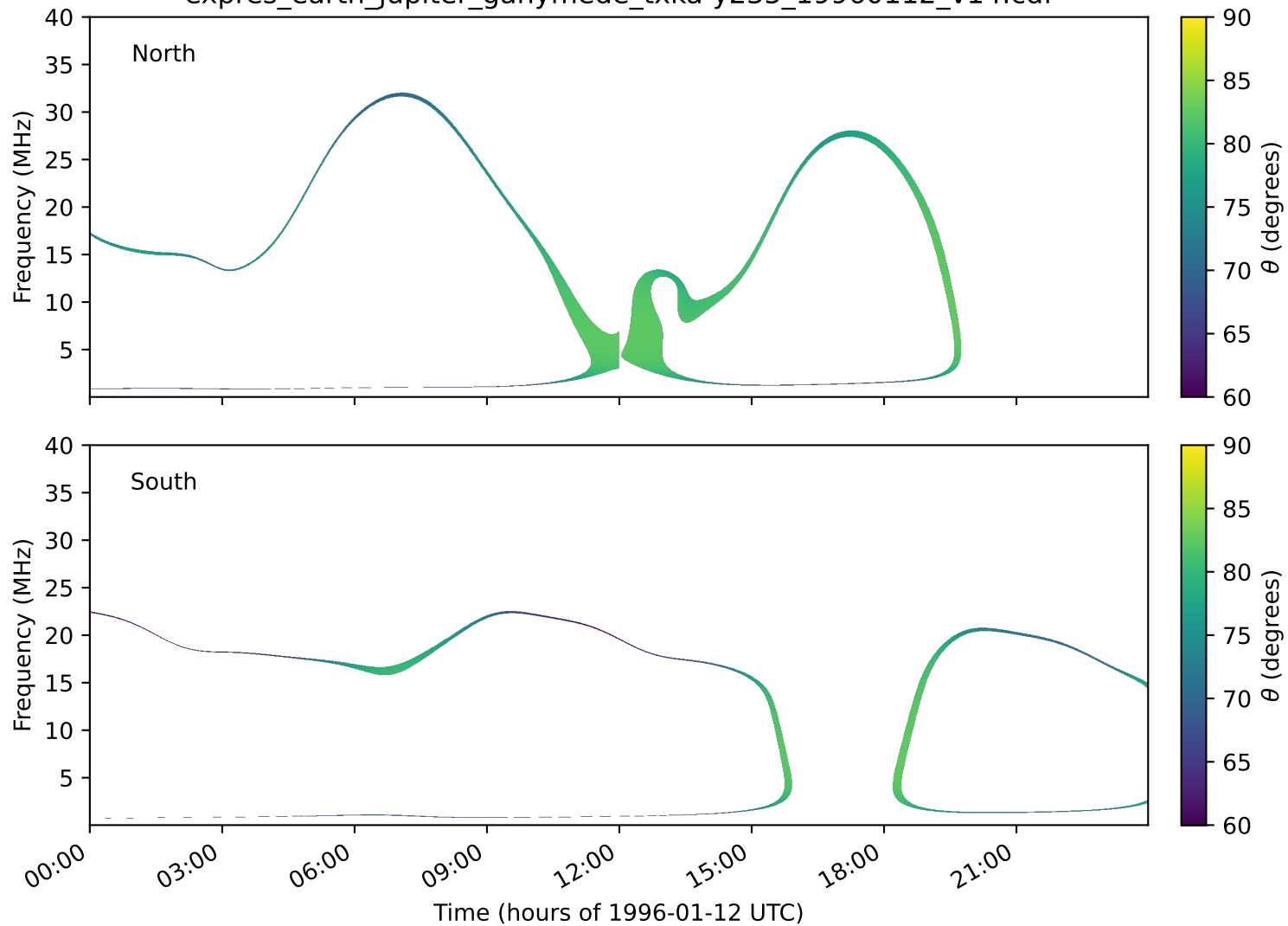
expres_earth_jupiter_ganymede_txka-y235_19960112_v14.cdf
